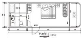
Model: S23 Length: 9.6m width: 3.3m height: 3.08m Building area: 32m
