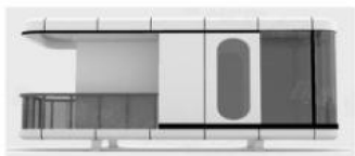
Model: B21 Length: 8m width: 3m height: 3m Building area: 24m 2
