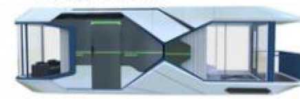
Model: A42 Length: 11.5m width: 3.3m height: 3.3m building area: 38m'
