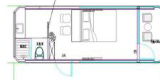
Model: A53 Length: 8.5m width: 3.3m height: 3.2m. Building area: 28m 2
