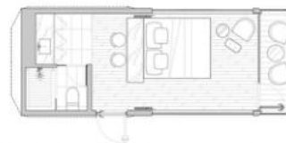
Model: S22 Length: 9.1m width: 3.3m height: 3.3m. Building area: 30m
