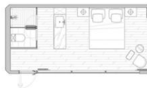
Model: B11 Length: 7.5m, width: 3.3m and height: 3.2m. Building area: 24.751g.
