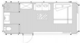
Model: A21 Length: 7.5m, width: 3.3m and height: 3.2m. Building area: 25m 2
