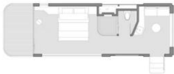
Model: B72 Length: 10.6m, width: 3.2m and height: 3.2m. Building area: 34m 2
