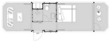
Model: A23 Length: 11.5m, width: 3.3m and height: 3.2m. Building area: 38m 2
