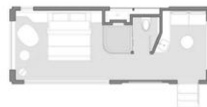
Model: B71 Length: 8.5m, width: 3.2m and height: 3.2m. Building area: 27.2m 2
