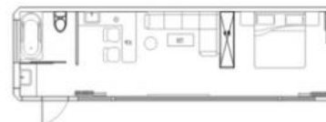
Model: B22 Length: 11.5m, width: 3.3m and height: 3.2m. Building area: 38m 2
